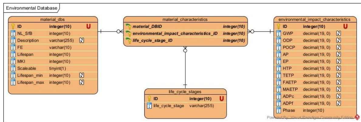
Figure 5.2: ERD diagram of material database
